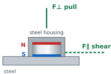
Single-sided pot magnet in steel housing F⊥ pull: 48,40 kg F∥ shear: 14,52 kg
