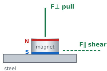
Bare magnet magnet without housing F⊥ pull: 19,36 kg F∥ shear: 5,81 kg
