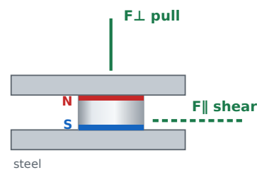
Double-sided pot two magnets, shared housing F⊥ pull: 1,86 kg F∥ shear: 0,56 kg
