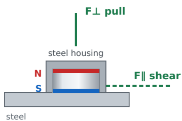
Single-sided pot magnet in steel housing F⊥ pull: 2,06 kg F∥ shear: 0,62 kg
