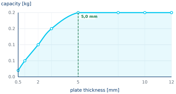
Steel thickness effect curve
