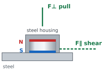
Single-sided pot magnet in steel housing F⊥ pull: 2,30 kg F∥ shear: 0,69 kg
