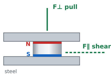
Double-sided pot two magnets, shared housing F⊥ pull: 2,07 kg F∥ shear: 0,62 kg
