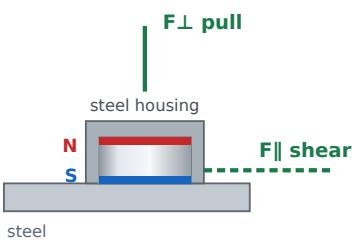
Single-sided pot magnet in steel housing F⊥ pull: 109,61 kg F∥ shear: 32,88 kg
