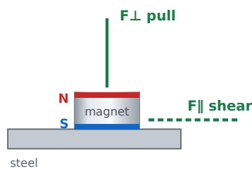
Bare magnet magnet without housing F⊥ pull: 0,23 kg F∥ shear: 0,07 kg
