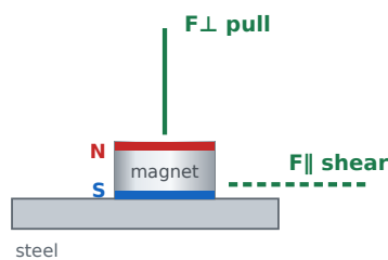
Bare magnet magnet without housing F⊥ pull: 7,73 kg F∥ shear: 2,32 kg
