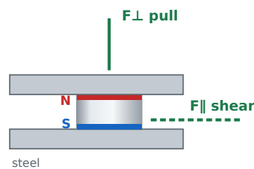
Double-sided pot two magnets, shared housing F⊥ pull: 17,12 kg F∥ shear: 5,14 kg
