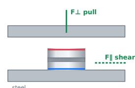
Double-sided pot two magnets, shared housing F⊥ pull: 16,33 kg F∥ shear: 4,90 kg
