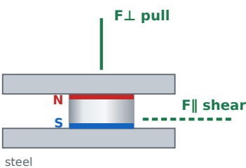
Double-sided pot two magnets, shared housing F⊥ pull: 3,69 kg F∥ shear: 1,11 kg
