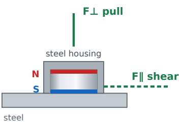
Single-sided pot magnet in steel housing F⊥ pull: 4,11 kg F∥ shear: 1,23 kg
