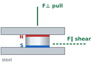
Double-sided pot two magnets, shared housing F⊥ pull: 122,44 kg F∥ shear: 36,73 kg
