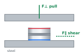
Double-sided pot two magnets, shared housing F ⊥ pull: 1,28 kg F ∥ shear: 0,38 kg
