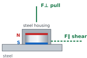
Single-sided pot magnet in steel housing F⊥ pull: 58,56 kg F∥ shear: 17,57 kg
