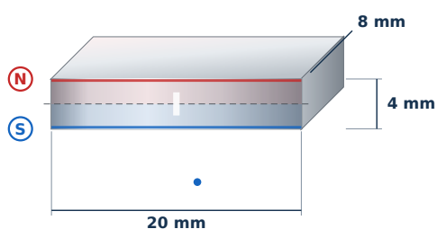
magnetization (S → N)
