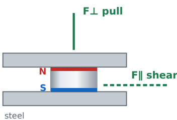
Double-sided pot two magnets, shared housing F⊥ pull: 221,00 kg F∥ shear: 66,30 kg
